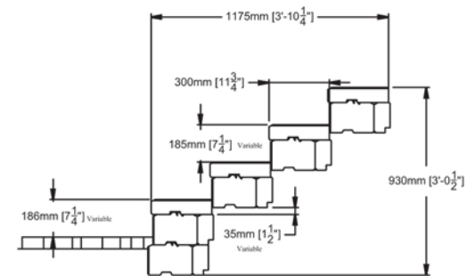
Ortana 12" Step Tread With Standard Unit
